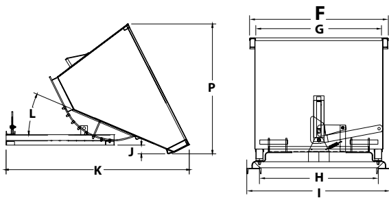
2, 2-1/2 cubic yard hoppers
