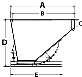
2, 2-1/2 cubic yard hoppers
